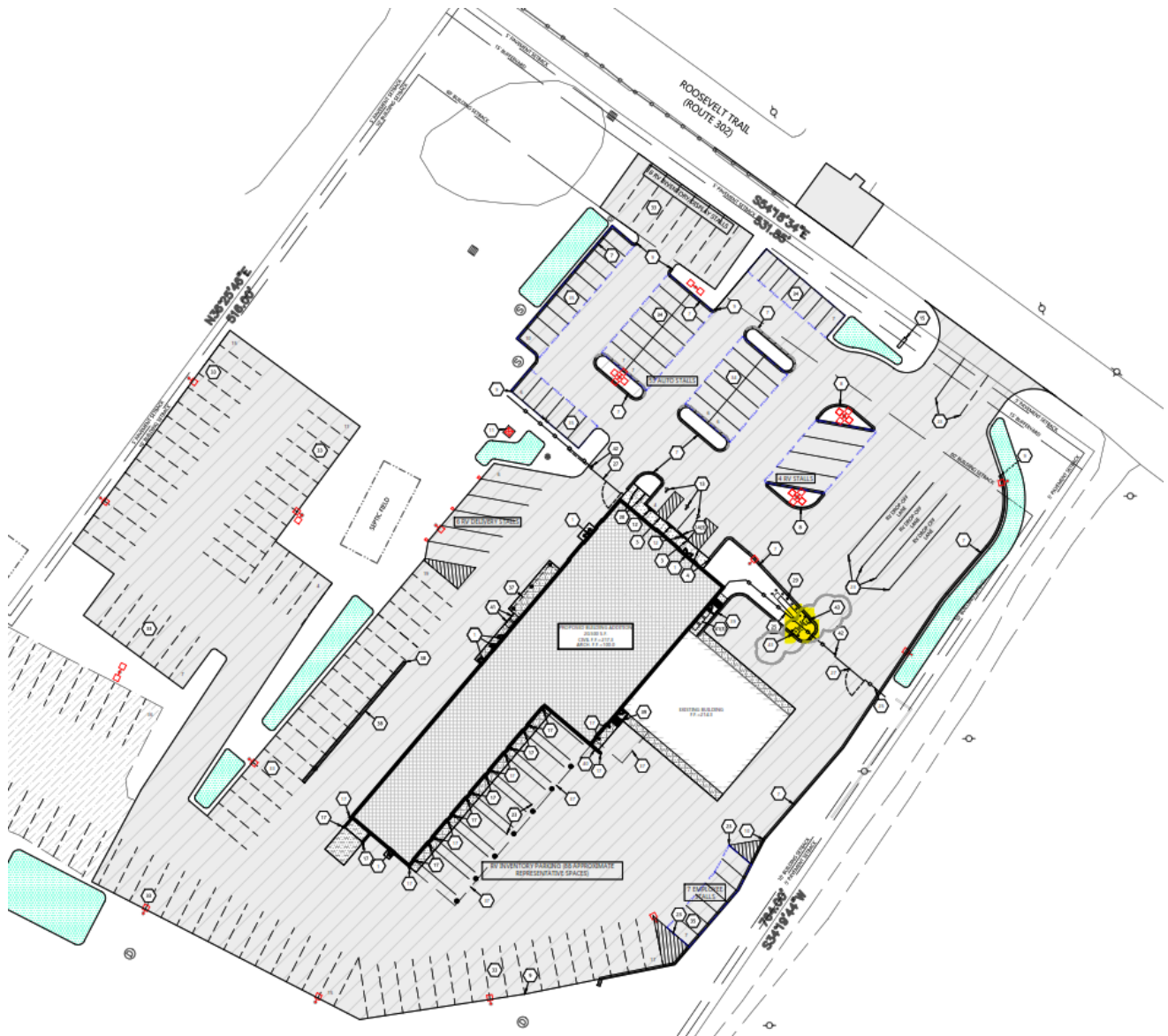
Figure 2. Approved Site Plan with proposed dump station location highlighted.
