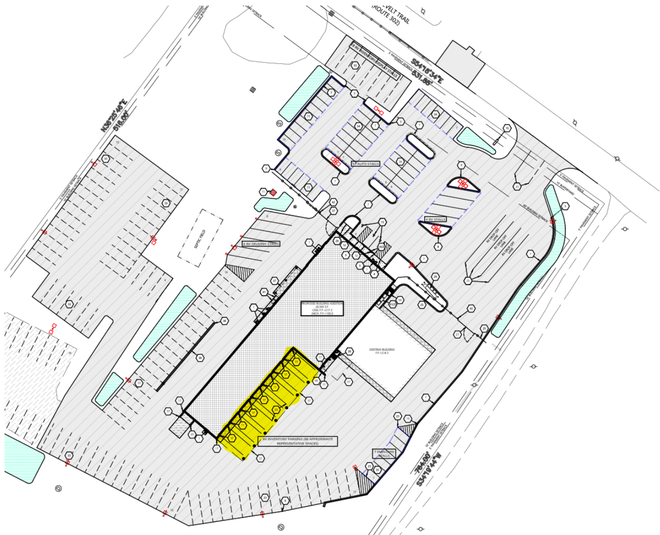
Figure 2. Approved Site Plan with proposed canopy addition highlighted.
