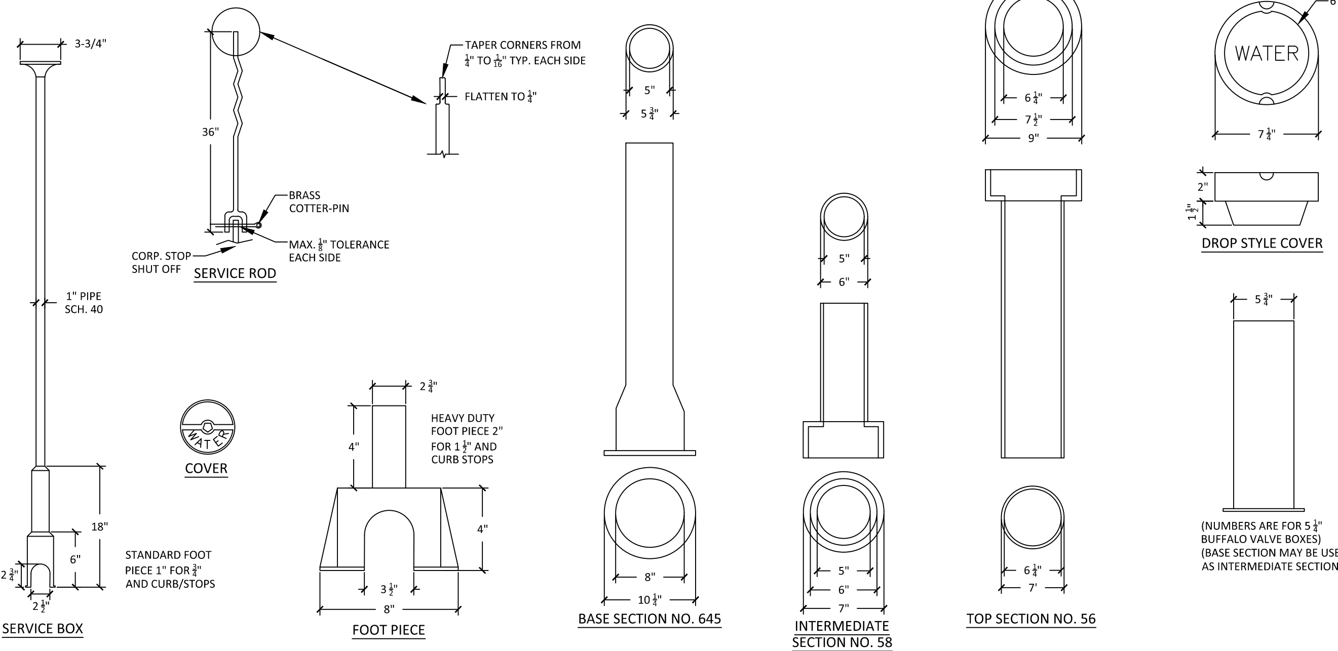
VALVE BOX & COVER NOT TO SCALE
