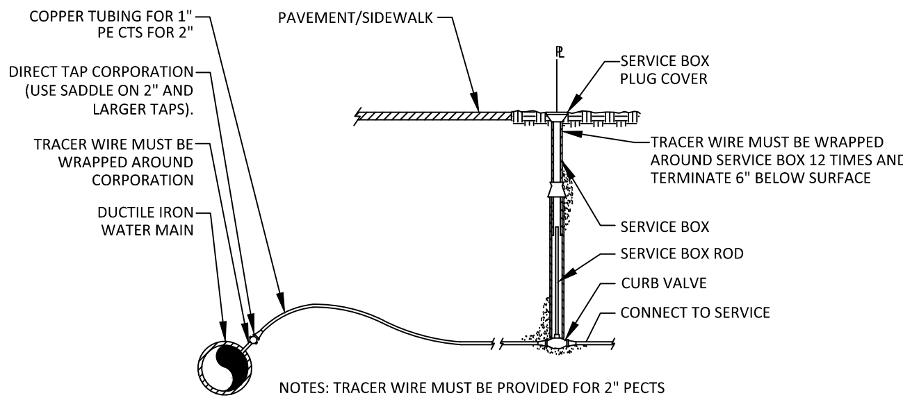
SERVICE DETAIL NOT TO SCALE
