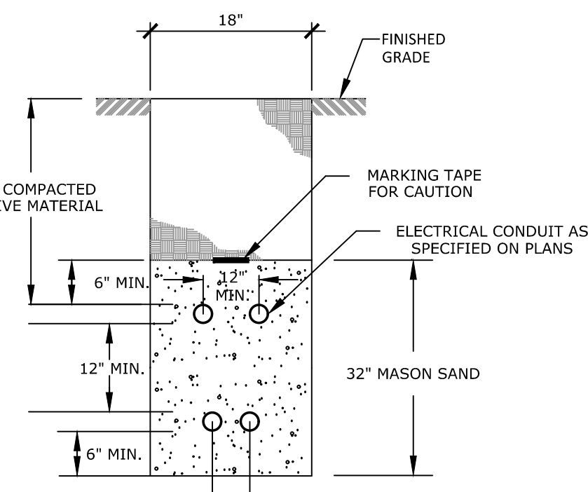
TRENCH DETAIL - ELECTRICAL CONDUIT NOT TO SCALE
