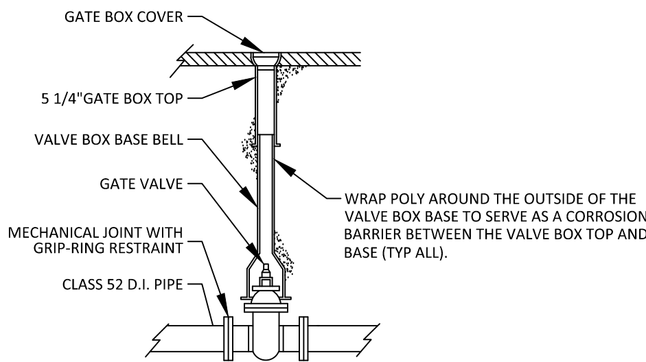
GATE VALVE NOT TO SCALE
