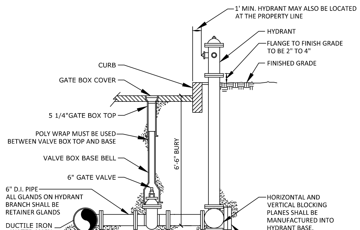
FIRE HYDRANT NOT TO SCALE
