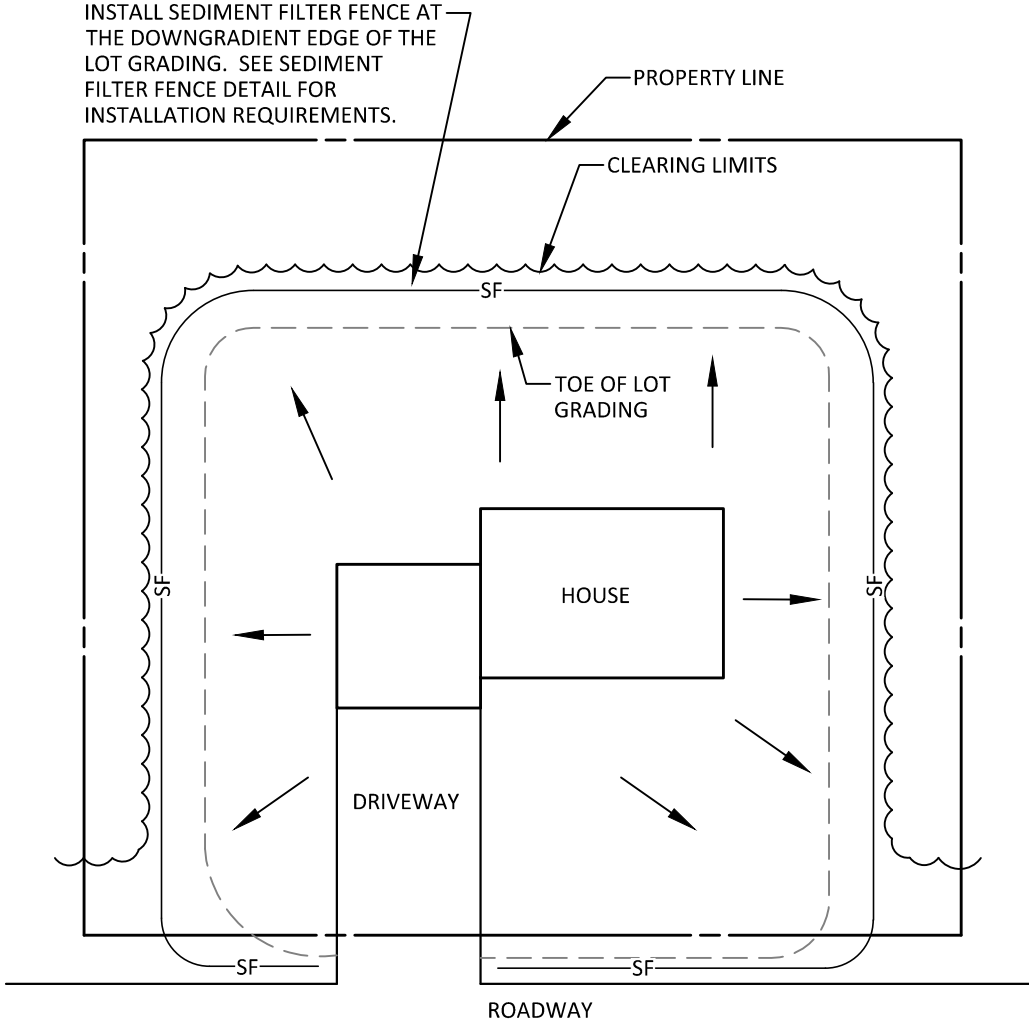
TYPICAL HOUSE LOT EROSION CONTROL DETAIL
